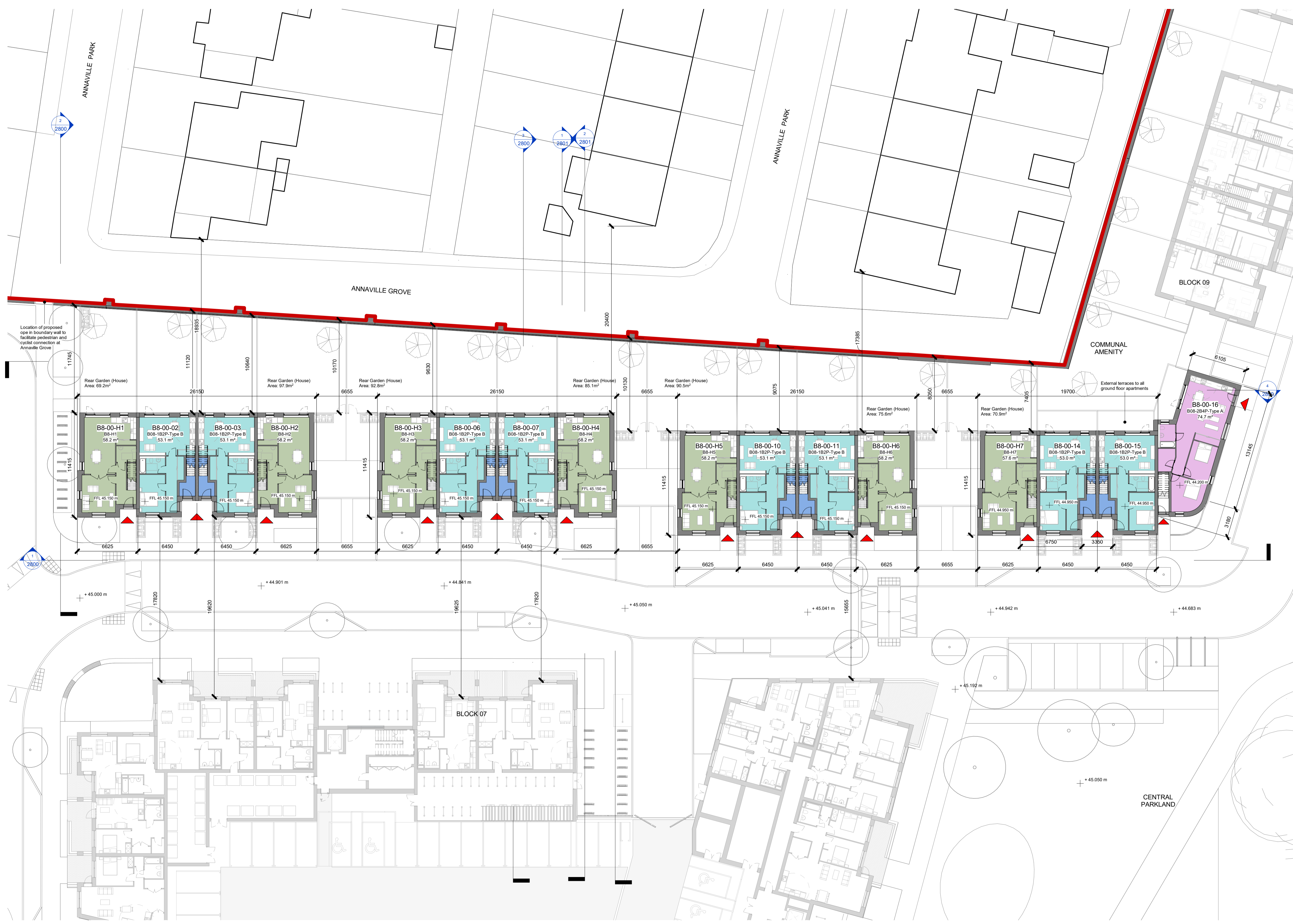
B8_00 - Ground Floor Plan 1 : 200
